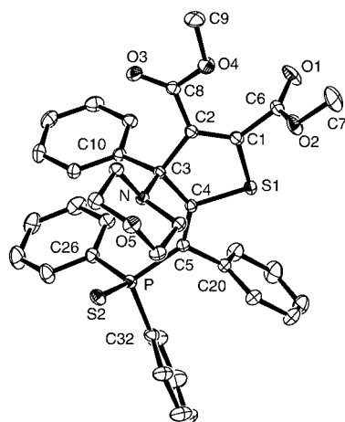
Figure 3. Structure of 18 in the crystal (ORTEP plot); ellipsoids of thermal vibration are shown at the 20% probability level; hydrogen atoms are not shown; selected bond lengths [Å] and angles [°]: C1–C2 1.332(5), C2–C3 1.535(5), C3–C4 1.566(5), C4–C5 1.353(5), C5–P 1.840(3), P–S2 1.949(1); C1–S1–C4 92.4(2), C3–C4–C5 134.1(3), S1–C4–C5 115.2(2), C4–C5–P 130.2(2), C4–C5–C20 116.2(3)
