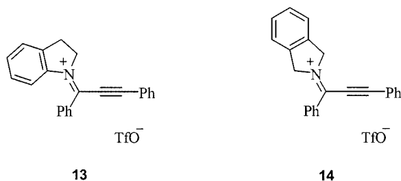
Scheme 5. Isomeric propyne iminium salts displaying different regioselectivity for nucleophilic addition of Me_3Si-OPPh_2
