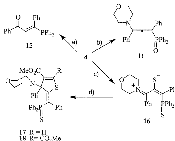
Scheme 6. Reagents and conditions: a) H_2O , acetone, 75% yield. b) (Me_3SiO)_2 , CH_2Cl_2 . c) S_8 , CH_2Cl_2 , 91%. d) RC\equiv CCO_2Me , 50^\circ C , 24 h ( R=H : 61%; R=CO_2Me : 41%)
