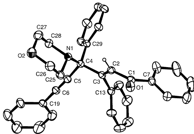
Figure 1. Structure of 10 in the crystal (ORTEP plot); ellipsoids of thermal vibration are shown at the 20% probability level; hydrogen atoms are omitted except for the olefinic H2; selected bond lengths [Å] and torsion angles [°]: C1–O1 1.222(2), C1–C2 1.483(3), C2–C3 1.332(2), C4–C5 1.486(3), C5–C6 1.192(2); O1–C1–C2–C3 -130.4(2)
