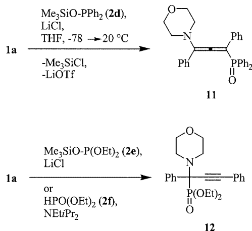
Scheme 4. Reaction between propyne iminium salt 1a and an O -silyl phosphonite or phosphite
