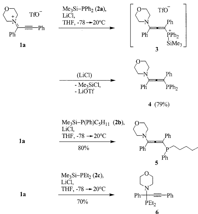
Scheme 1. Reaction between propyne iminium salt 1a and phosphanes Me 3 Si-PR 2
