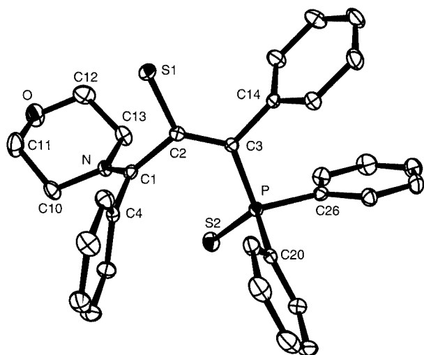
Figure 2. Structure of 16 in the crystal (ORTEP plot); ellipsoids of thermal vibration are shown at the 20% probability level; hydrogen atoms are not shown; selected bond lengths [Å] and angles [°]: C1–N 1.310(2), C1–C2 1.488(3), C2–C3 1.354(3), C3–P 1.803(2), C2–S1 1.715(2), P–S2 1.960(1); C1–C2–C3 126.4(2), C1–C2–S1 106.1(1), C3–C2–S1 127.4(1), C2–C3–P 123.5(1); torsion angles [°]: N–C1–C2–S1 83.1(2), C4–C1–C2–C3 82.6(2), C2–C3–P–S2 36.0(2)
