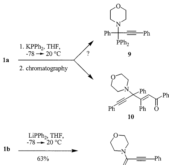
Scheme 3. Reaction between propyne iminium salts 1a and 1b and potassium (or lithium) diphenylphosphide
