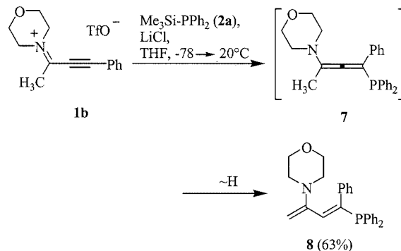
Scheme 2. Formation of a 2-dienamine from propyne iminium salt 1b
